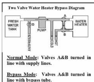
Two Valve Water Heater Bypass
